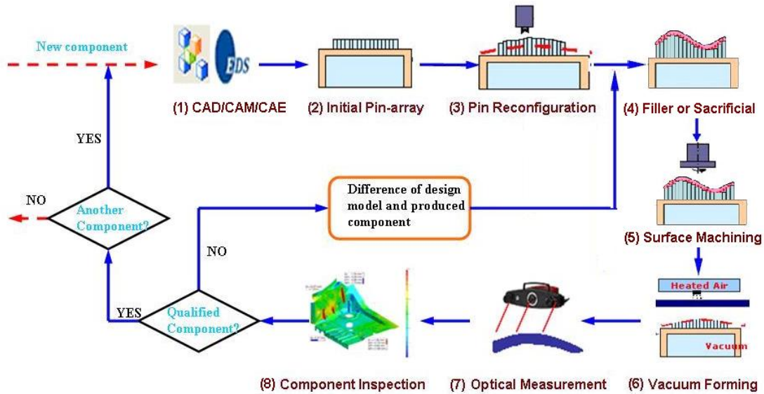
Fig.1 Development architecture of the HAVES test bed
